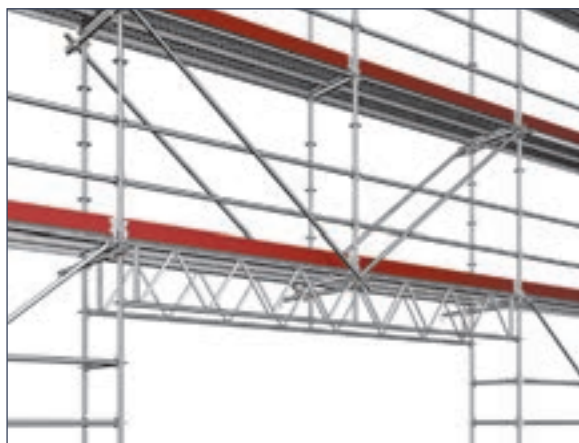
Installation situation: Spigot and U-ledger
