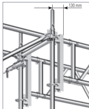
GI connection 0.5 m, with 2 wedge-heads
